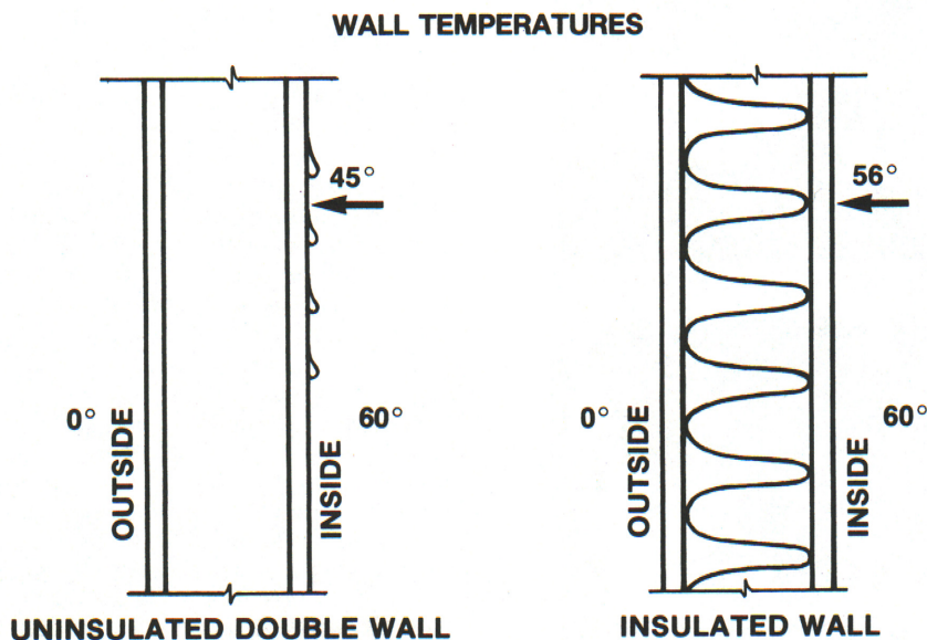
Figure 1. Insulation can make a difference in whether or not condensation occurs on inside wall surfaces. With wall temperatures of 0 F. outside and 60 F. inside and with relative humidity of 75%, condensation starts at 53 F.
