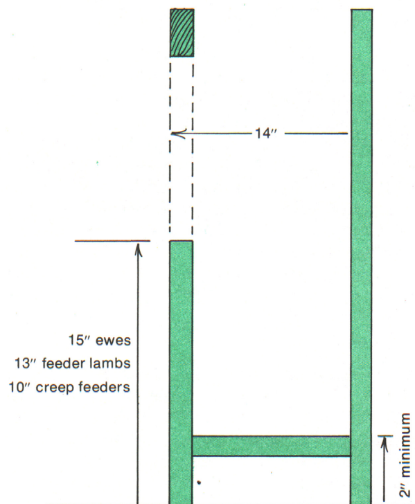
Fig. 6—Typical feeder for feeding on one side.
