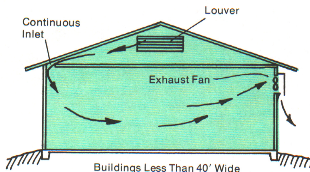
Fig. 9—Mechanical ventilation example.
