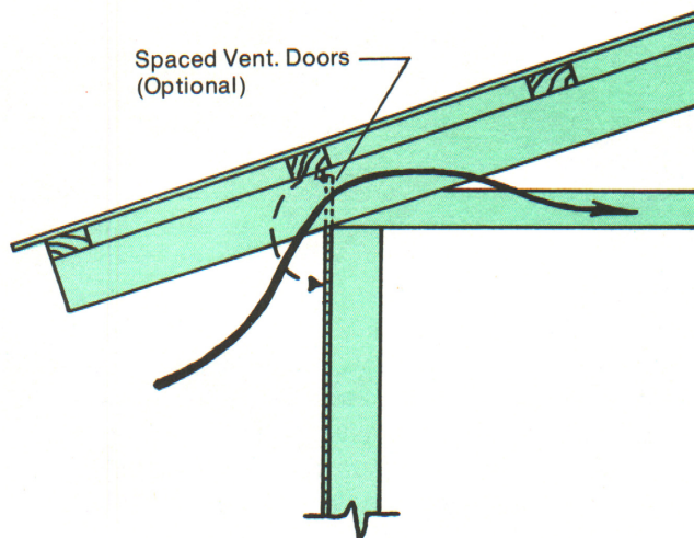
Fig. 8—Under-eave air inlet.
