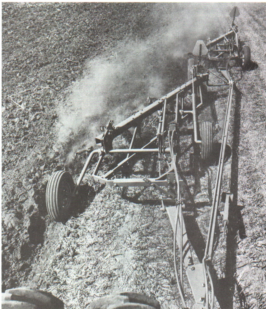
Figure 5 —Modern, tandem moldboard plow used on dry soil to increase rain water infiltration rates and to loosen a compacted soil. Dual wheels of tractor are on-land rather than in-furrow, which is desirable when working soil with more moisture. With the modern, high-clearance moldboard plow, there is little need to disc or chop crop residues before plowing.
