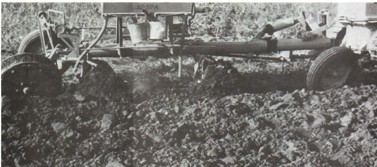
Figure 4 —Giant disc plow used in Michigan research program. Penetration to 30 inches was possible. This plow was modified for application of fertilizer and lime as plow down treatments. While this plow was designed with four discs, only two were used because of inadequate power. Deep plowing is the only known way of improving the soil conditions described in Figure 1.
