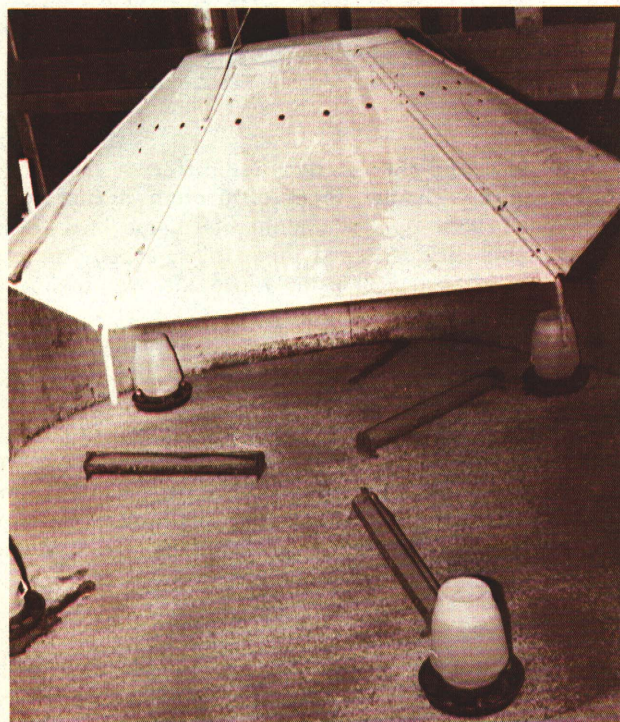
Figure 6. Suggested brooding area to start birds. (Hover was raised to take picture.)
