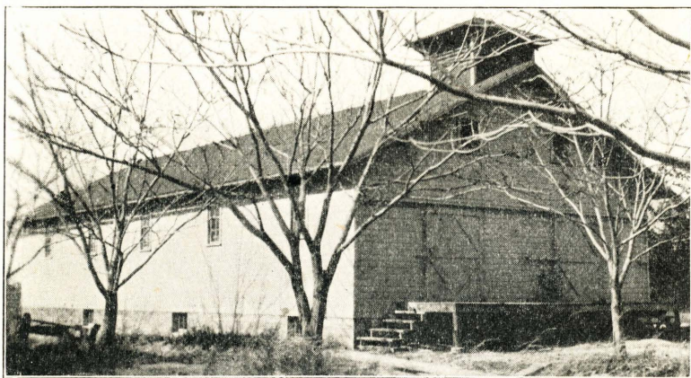
Fig. 26.—Storage R. See Table 2 for description. The basement of this combination packing and storage house is used for storing fruit. In addition to the basement windows, which may serve as cold air intakes, there are five intakes at the farther end of the building, near the storage room floor.
