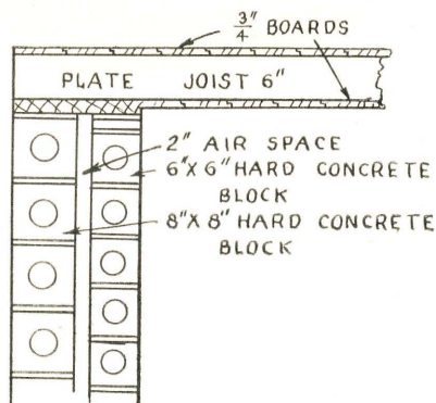
Fig. 22.—Detail of wall and ceiling construction of Storage G.
