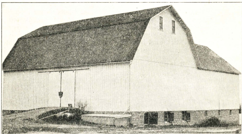
Fig. 30.—Storage H. One corner of this large barn basement was partitioned off and insulated. It has not proved a satisfactory storage for two reasons: (1) there are neither outlet flues nor provision for taking advantage of wind because of the three air openings are all on the same side of the room, and (2) it has been almost impossible to maintain the humidity high enough to prevent wilting. See Table 2 for description.
