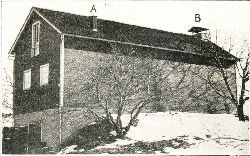
Fig. 12.—Storage B. See Table 2 for description. The forcing of air through an underground tile by means of a fan and releasing the warm air through the small ventilator at A was discontinued in 1923, when the larger ventilator at B was constructed and the large front door was made to serve as the only air intake. The later results were much better.
