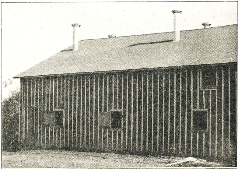
Fig. 29.—Storage C. A good storage was constructed in one end of this large barn. The original barn windows serve as cold air intakes. The four ventilating flues are too small to afford sufficient flow on still nights. See table 2 for description.
