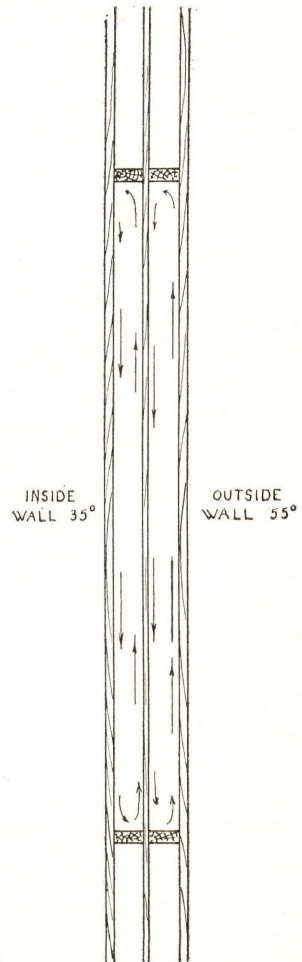
Fig. 7.—Illustrating heat transmission through hollow walls. The air in the right inclosed space, being heated by contact with the warmer boards, becomes lighter and rises; when it arrives at the top of the confined space, it passes down the right side of the middle board where it gives up its heat; as it is cooled, it contracts and becomes heavier, and sinks to the bottom of the inclosed space. In this manner, heat is transmitted from the outer board wall to the middle one, and in turn from the middle wall to the inner one.
