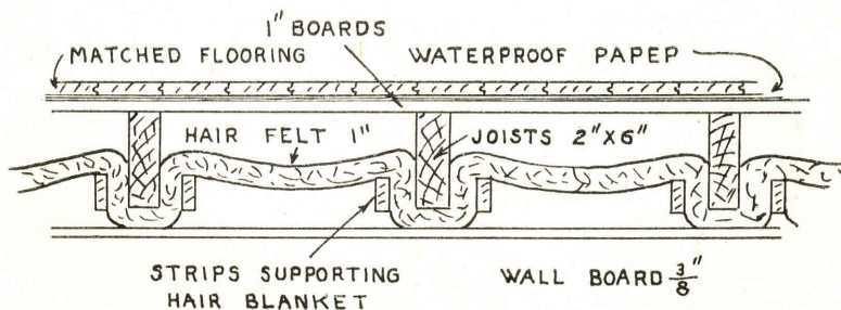
Fig. 18.—Detail of ceiling construction of Storage E.
