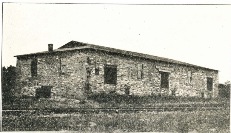
Fig. 28.—This combination packing house and basement storage is typical of many in operation in western New York. The basement windows, three of which are shown, are large and are usually located on opposite sides of the building. There are no outlet flues extending through the ceiling and roof. The wind blows into the storage room through the large openings on the windward side and passes out similar ones on the leeward side.
