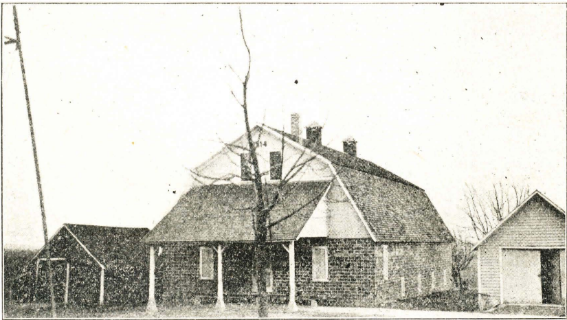
Fig. 8.—Storage A. See Table 2 for description and Figures 9 and 10 for details of construction. The depreciation of a house of this type is small.
