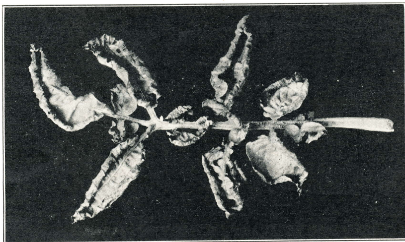
Fig. 28. Potato leaf, showing hopper-burn.
