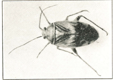
Fig. 4. Tarnished plant-bug, greatly enlarged.
