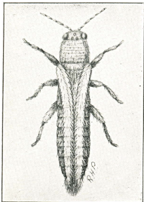
Fig. 12. Onion-thrips, greatly enlarged.
