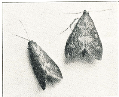
Fig. 47. Adult moths of European corn-borer, slightly enlarged.
