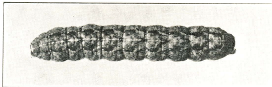
Fig. 6. Climbing cut-worm, Lampra alternata . Enlarged.
