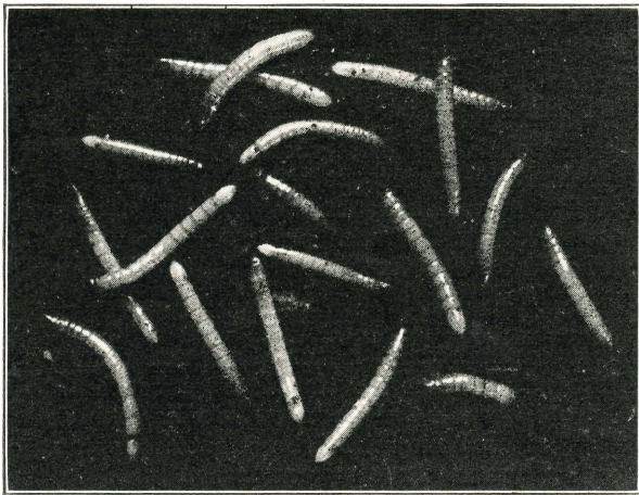
Fig. 55. Wire-worms, larvae of snapping-beetles.
