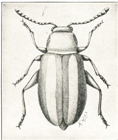
Fig. 17. Pale striped flea-beetle, enlarged.
