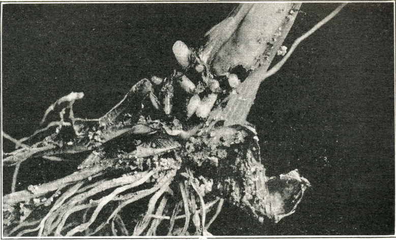
Fig. 10. Onion-maggot and its work in small onion, enlarged about twice.
