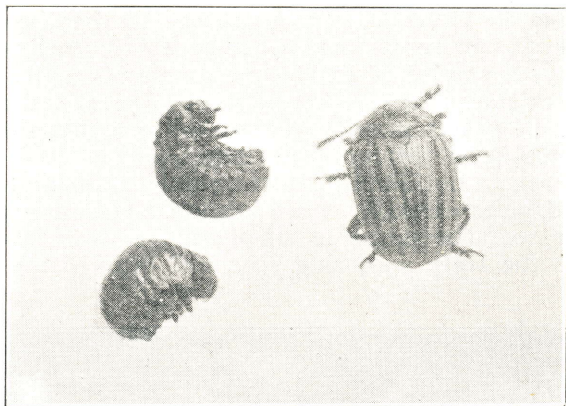
Fig. 29. Potato-beetle; adult beetle and larva, enlarged.
