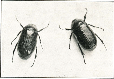
Fig. 54. June-beetles ( Phyllophaga fusca ).
