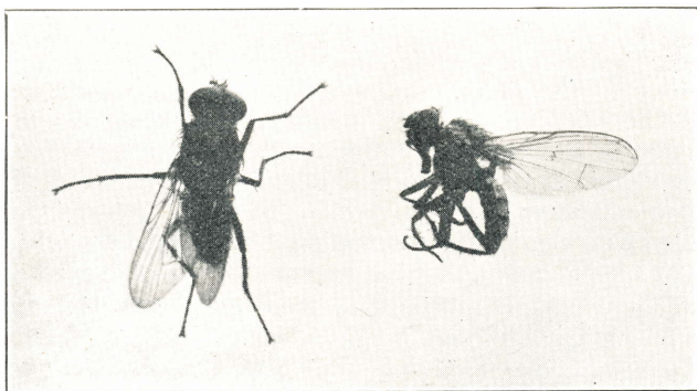
Fig. 32. Adult of bean maggot, enlarged about four times.
