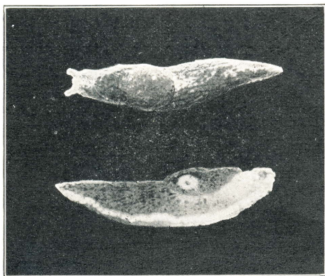
Fig. 23. Gray field slug, enlarged.
