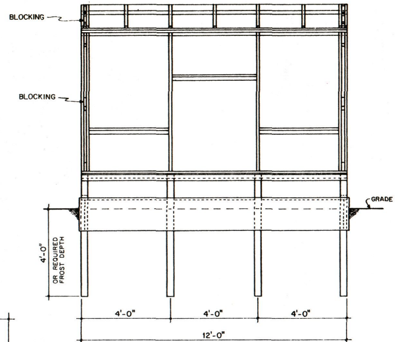
SOUTH WALL FRAMING
