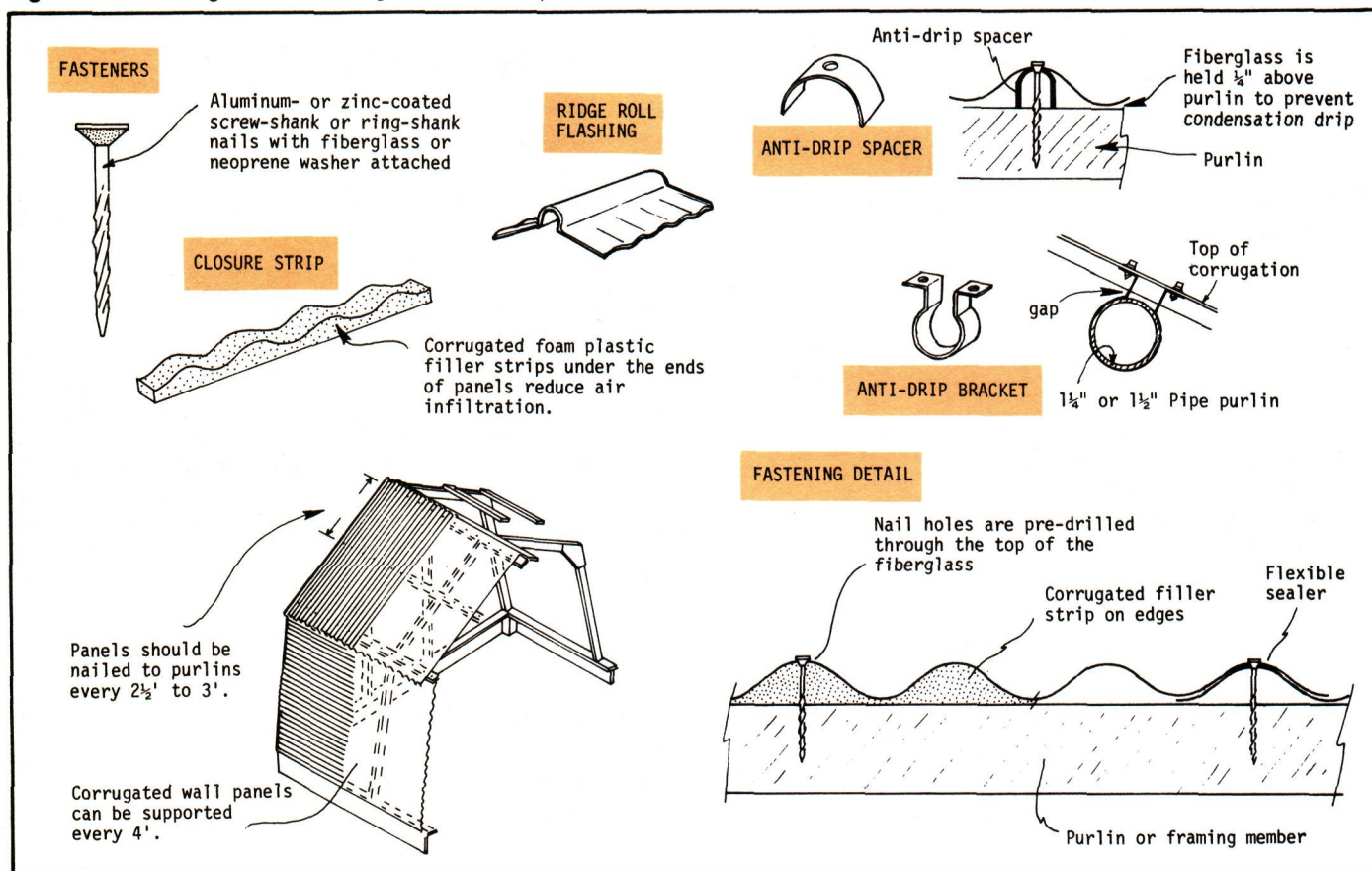
Figure 14. Fastening details for fiberglass reinforced panels
