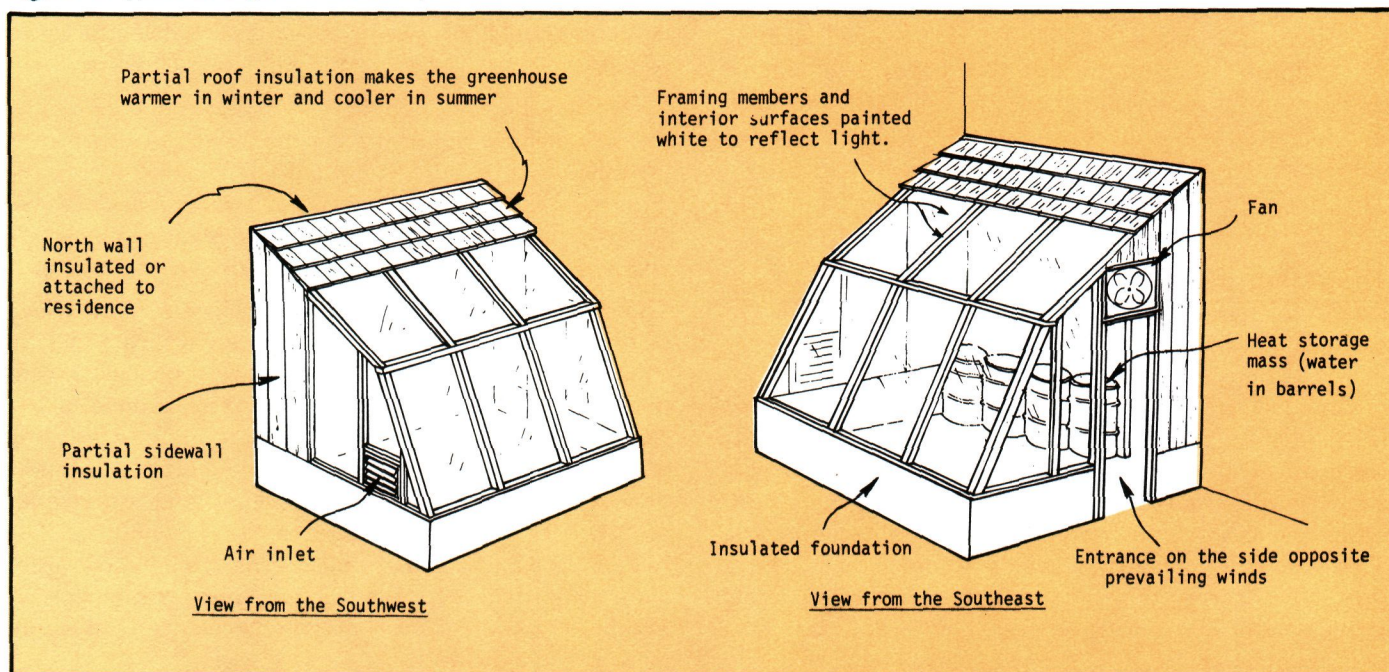
Figure 1. Typical solar greenhouse components
