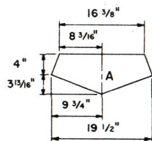
SIDE GUSSETS 16 REQ'D
