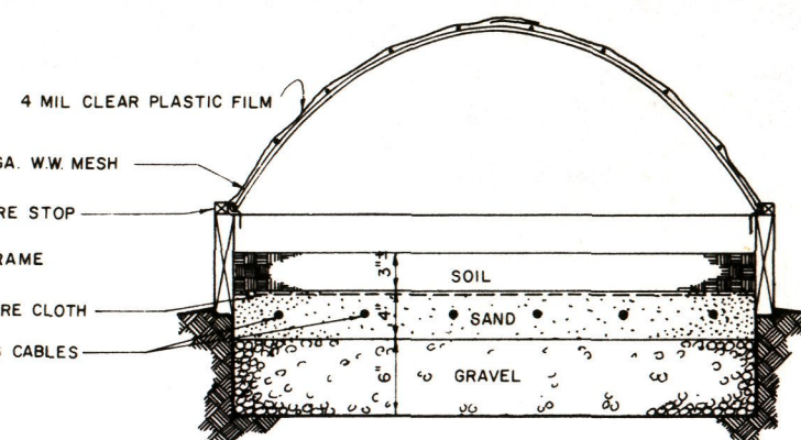
END VIEW SECTION
