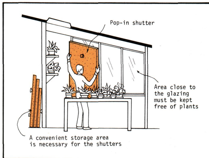
Figure 22. Pop-in shutters
