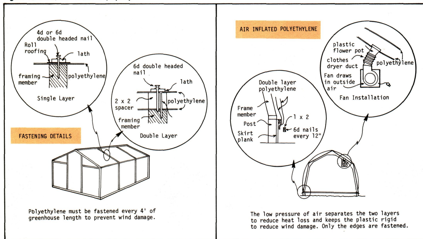
Figure 15. Installation details for polyethylene
