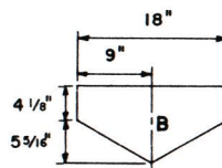
HEAD GUSSETS 8 REQ'D
