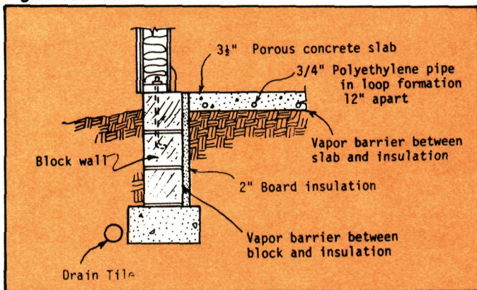
Figure 19. Detail of a heated floor
