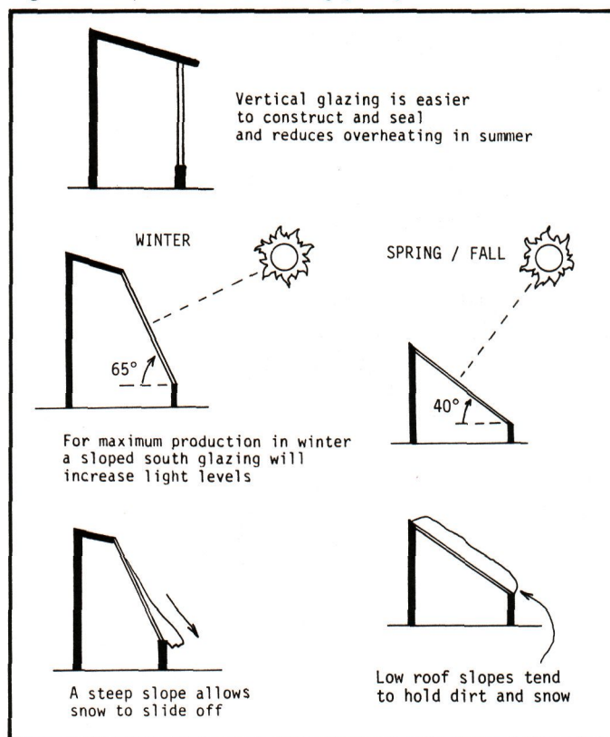
Figure 5. Slope of the south-facing glazing.
