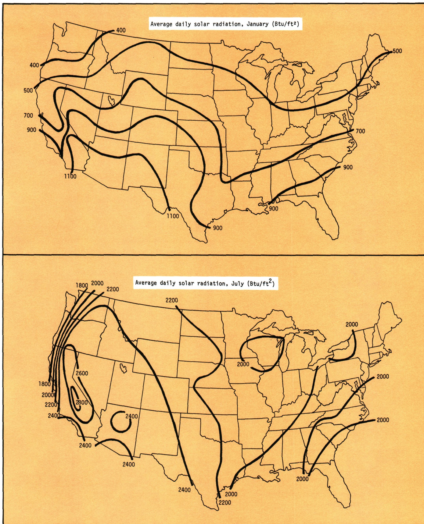
Figure 4. Solar radiation maps for January and July
