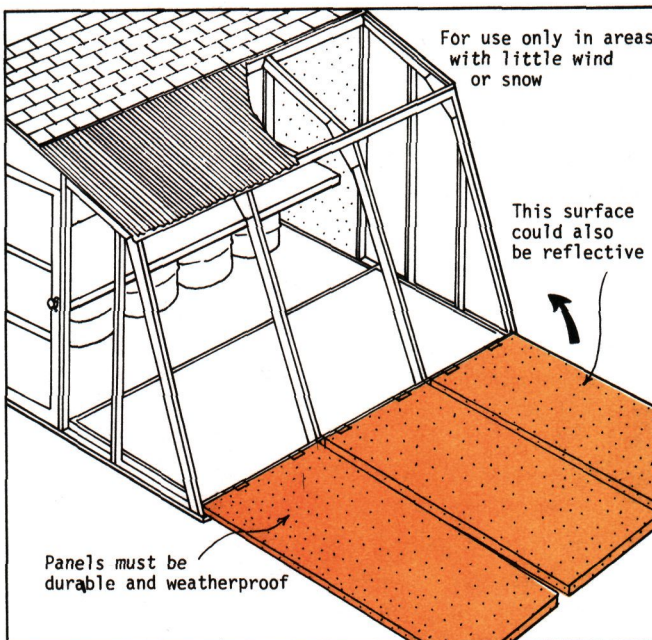
Figure 25. Exterior insulation system
