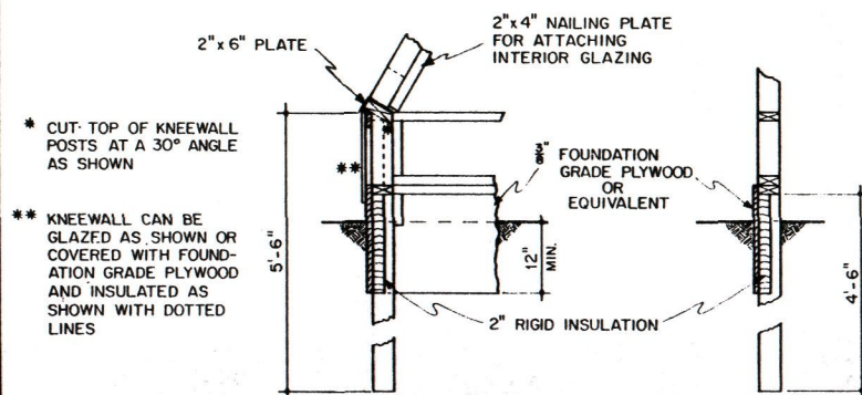
KNEEWALL AND FOUNDATION DETAILS
