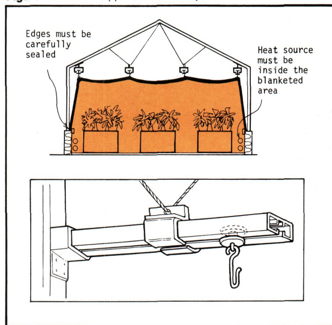
Figure 23. Track supported blanket system
