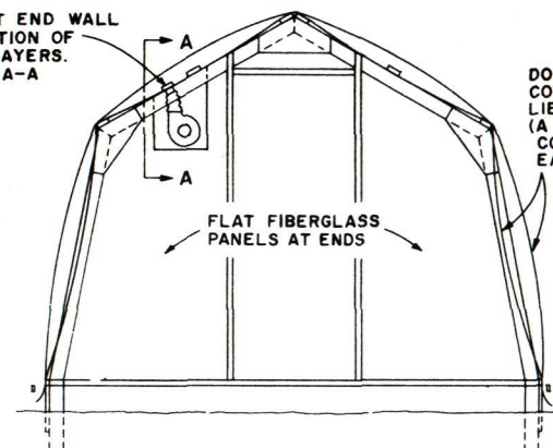
ALTERNATE CROSS SECTION
