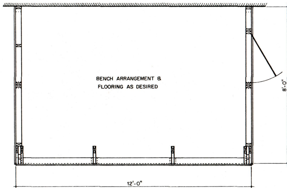
BASIC FLOOR PLAN LENGTH MAY BE EXPANDED IN 4' INCREMENTS SCALE: \frac{3}{8} " = 1'-0"
