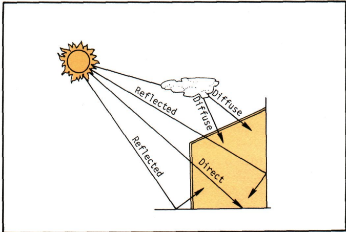
Figure 3. Types of solar radiation
