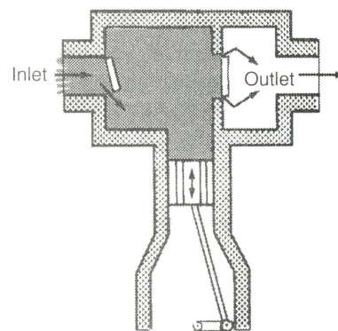
Piston pump.
